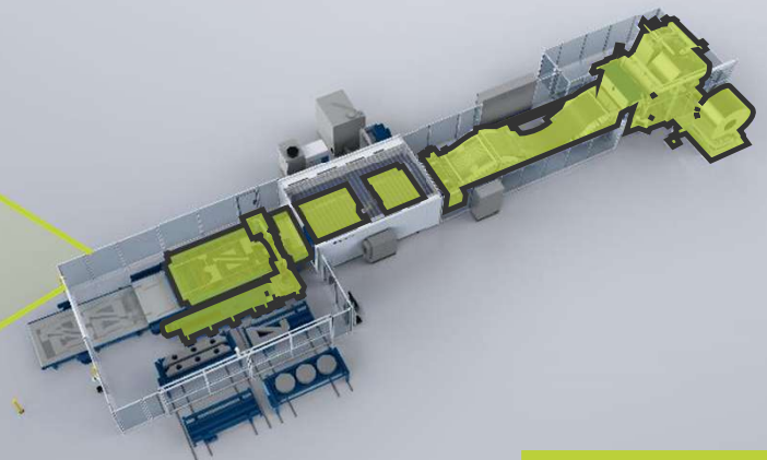
TruLaser 8000 Coil Edition (TC18)
